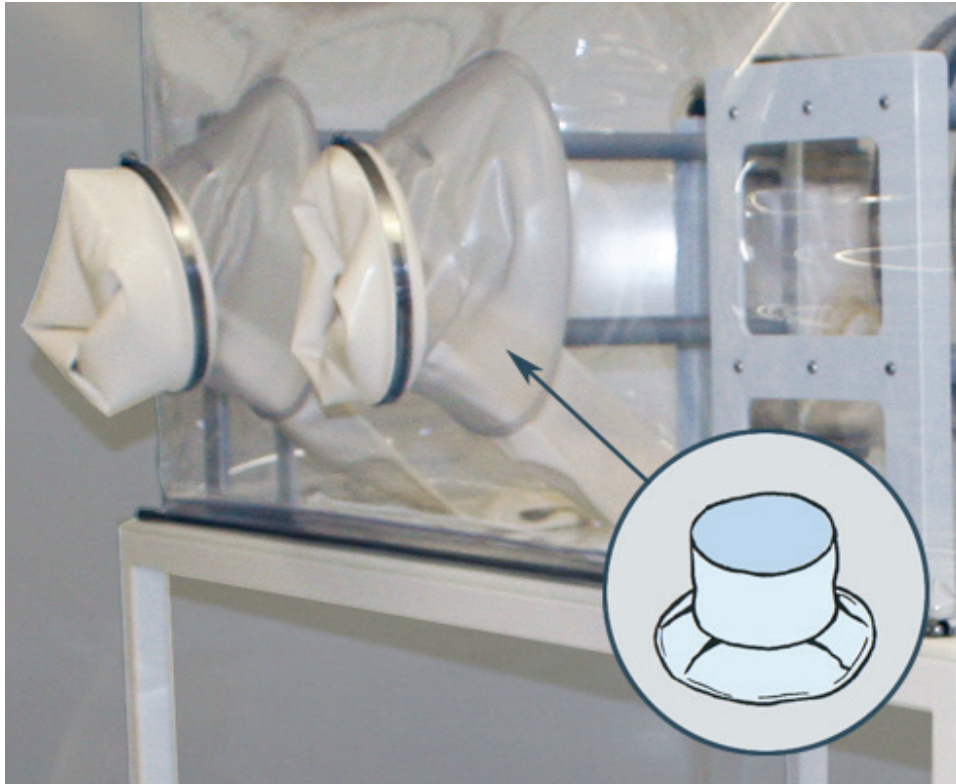
Pictured above are two 12" diameter/8" glove port Glove Extensions on a flexible film, positive pressure isolator system.
