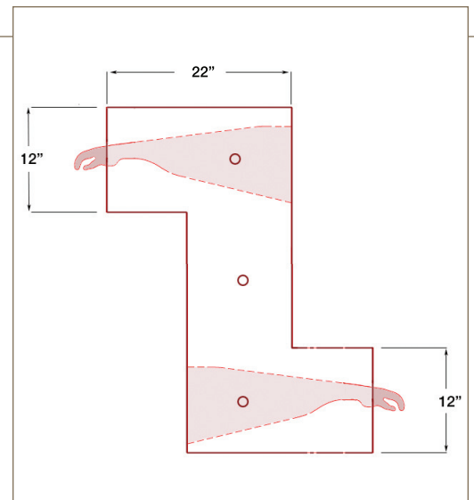
Above: A 2-tier "Z" transfer sleeve for tier-to-tier flexible film isolator connections between top canopy of a double-tier system and a lower tier canopy of a different isolator system.
