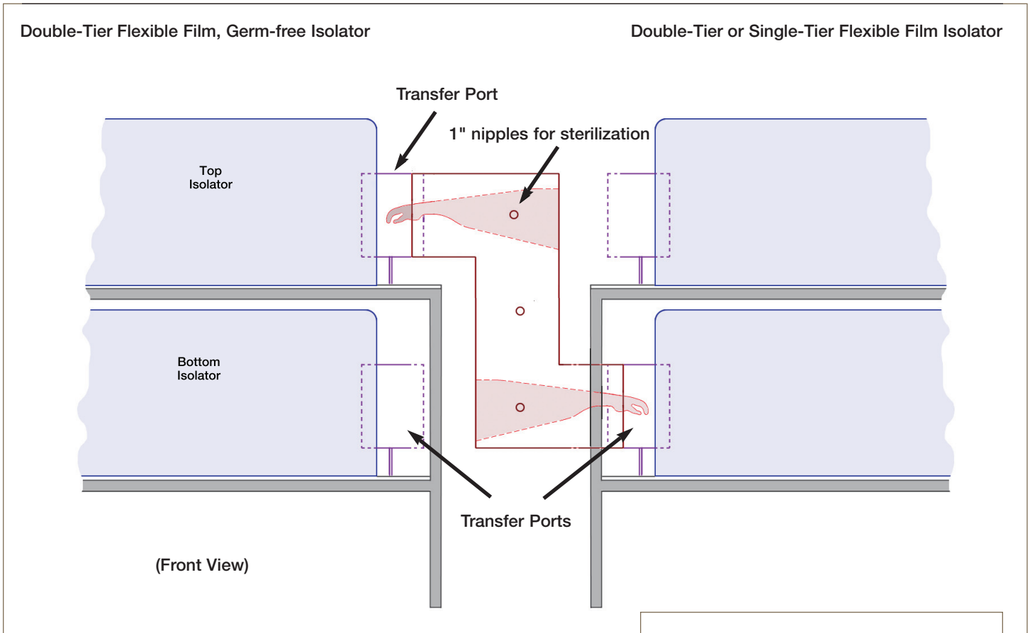
Above: A 2-tier "Z" transfer sleeve for tier-to-tier flexible film isolator connections between top canopy of a double-tier system and a lower tier canopy of a different isolator system.
